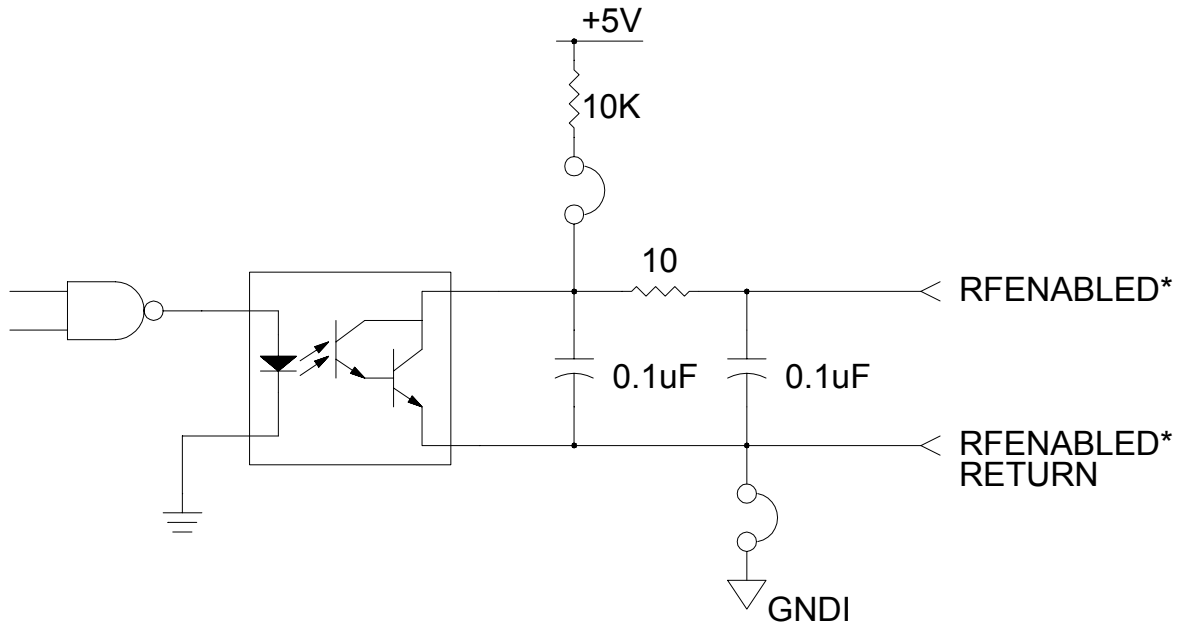
Figure 1: RFENABLED* Circuit
